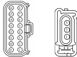
Headlight Harness Turn Signal Harness
