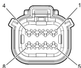
Headlight Connector
