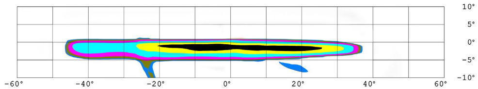
2018 Stock Mustang Combination Lamp Isolux
