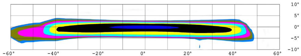
2018 Elite Series Mustang Combination Lamp Isolux
